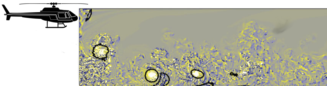
Instantaneous vorticity field generated by a helicopter hovering near the ground.
